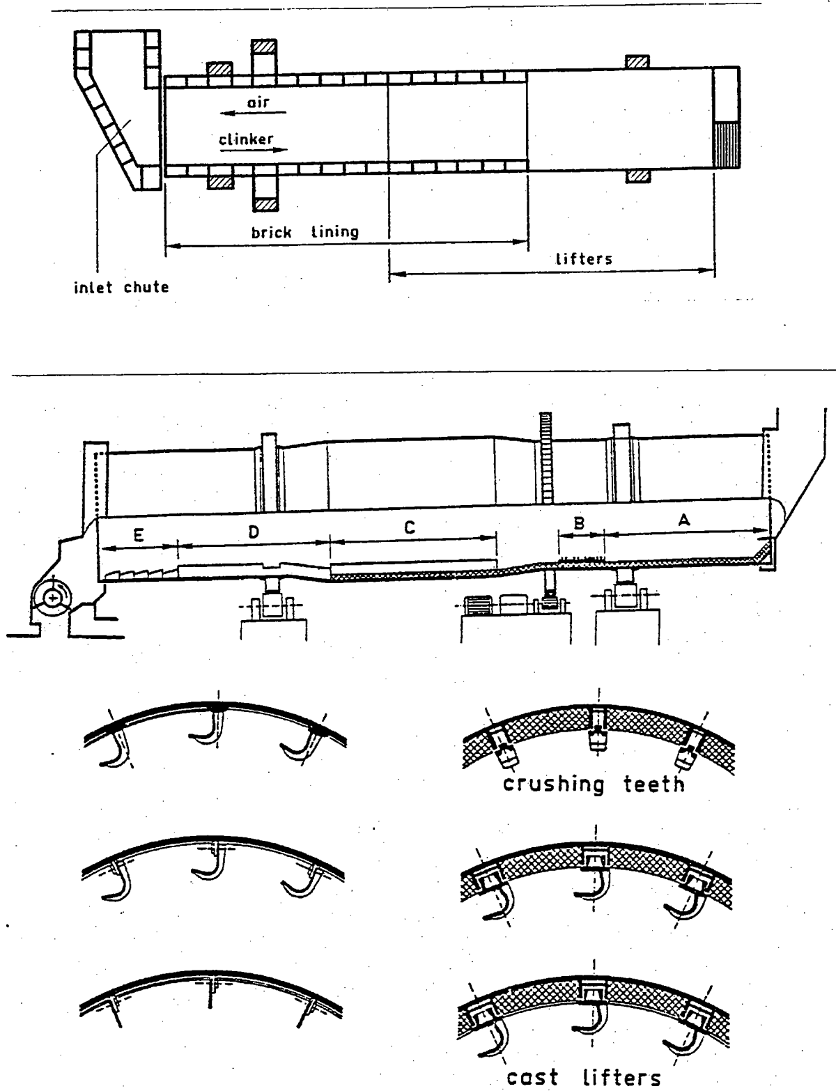
Figure 25 Rotary cooler
