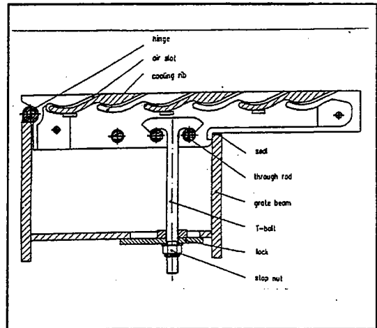
Fig.10d Controlled flow grate (Fuller) CFG plate
