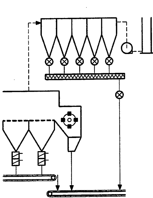
Multiclone
