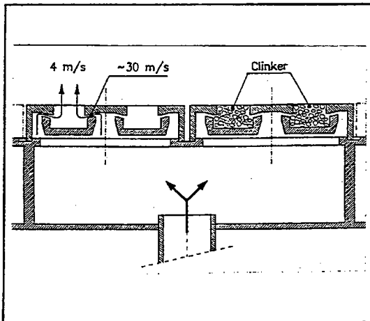
Fig.10e Jet ring plate (Polysius)
