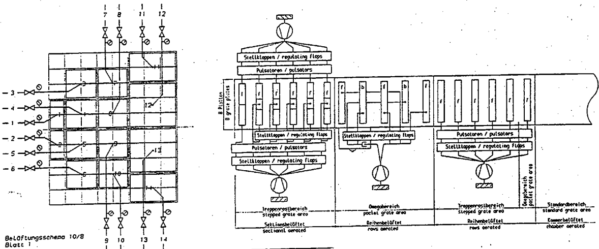
Figure 12 Aeration patterns
