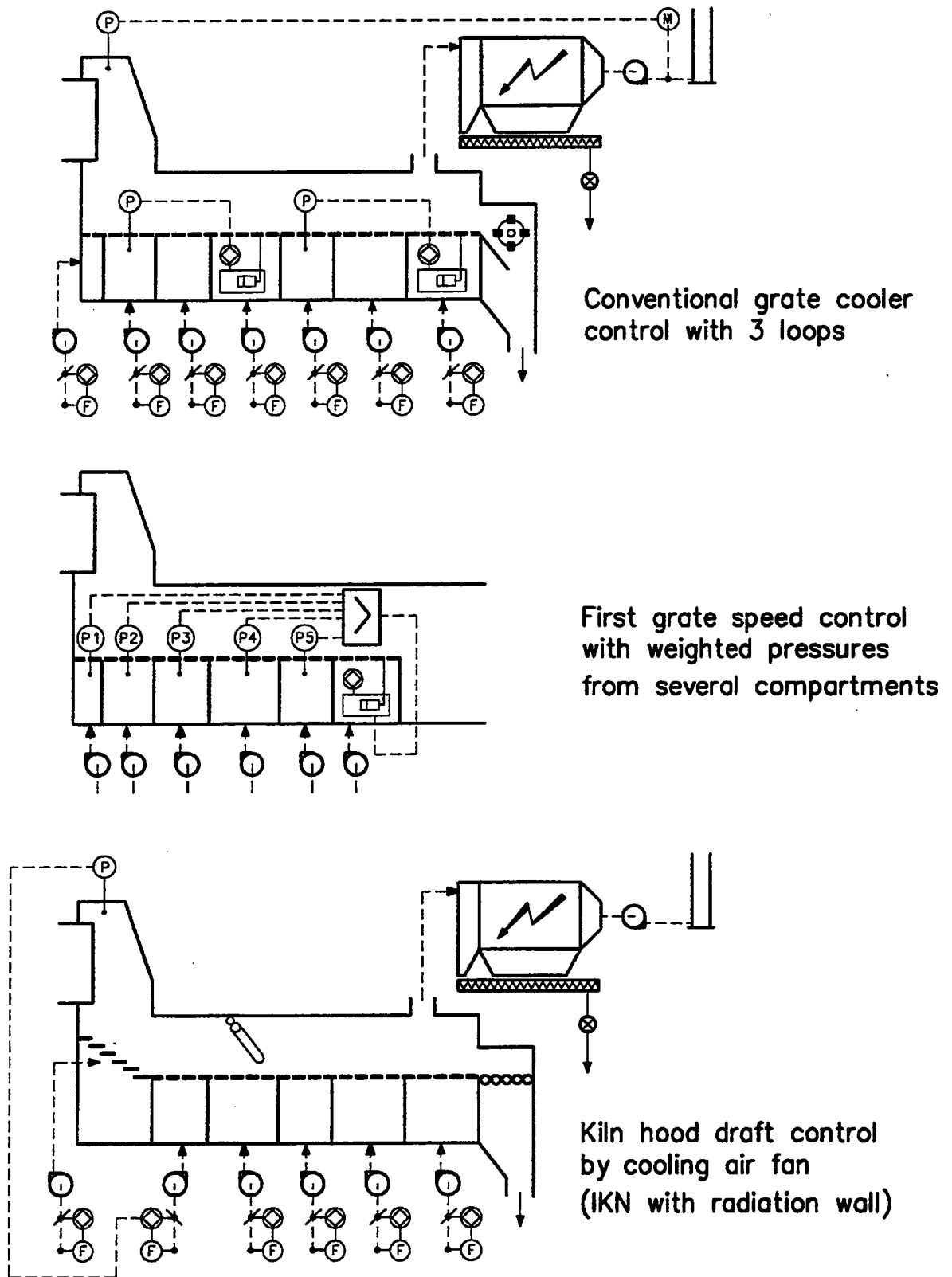
Figure 18 Cooler control
